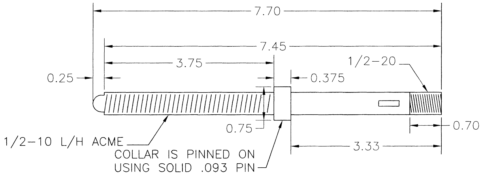
CLAUSING 5900 LATHE TAILSTOCK SCREW
