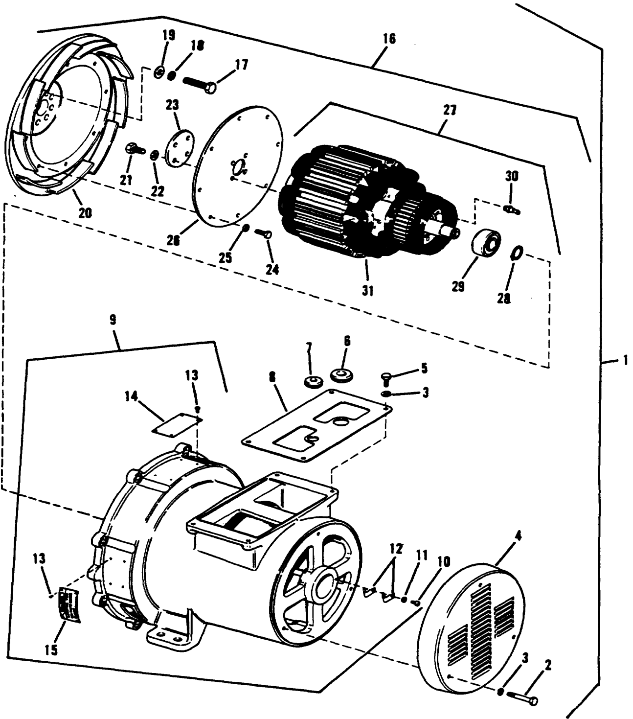
Figure 33. Generator Assembly (400 Hz), Group 03 (Electrical Power Generation System)
