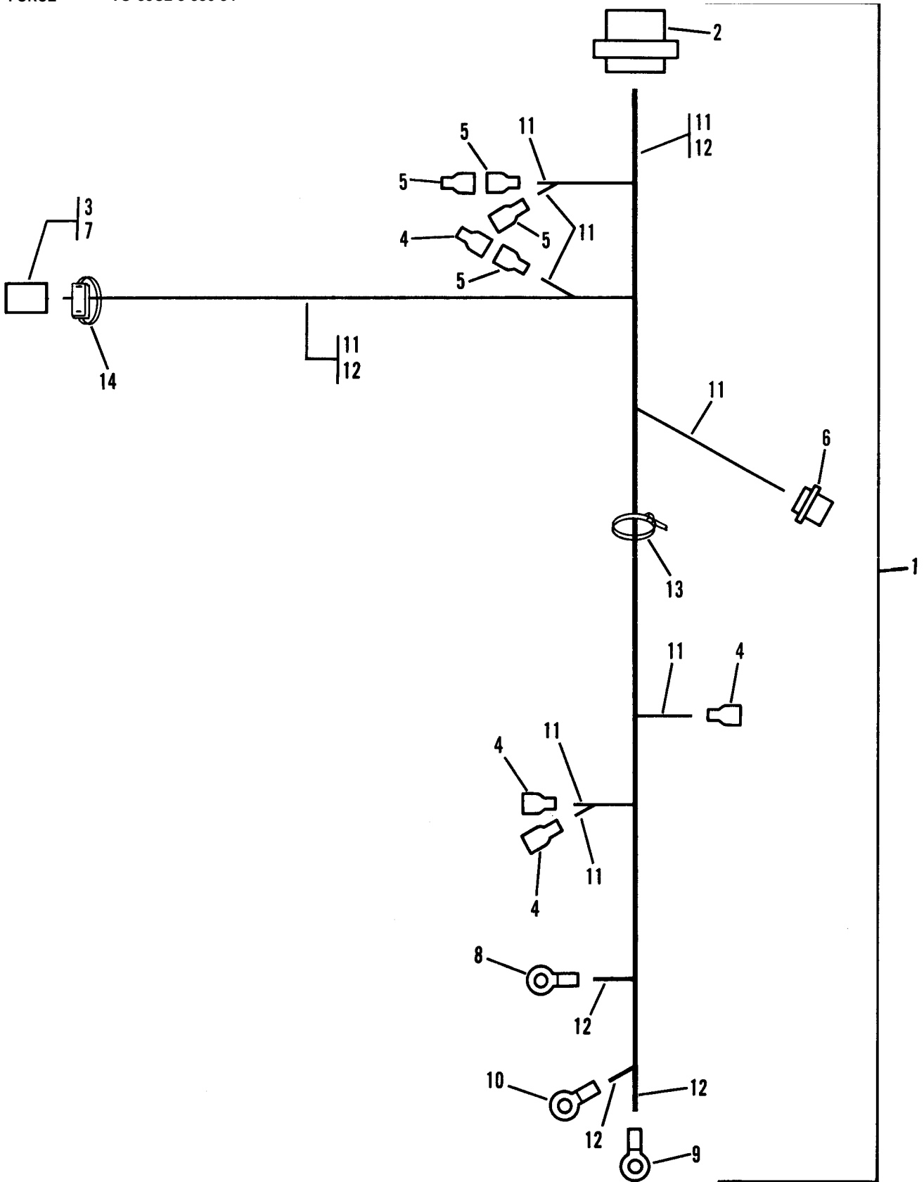
Figure 14. Engine Wiring Harness, Group 01 (DC Electrical and Control System)
