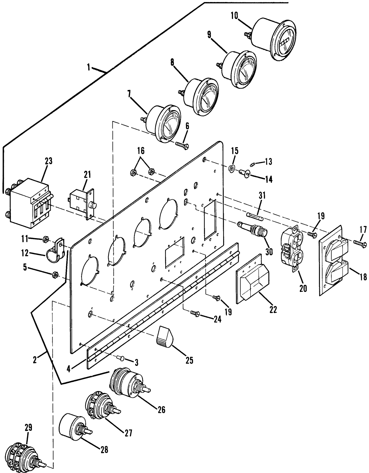
Figure 40. Meter Panel 60 Hz, Group 08 (Generator Controls and Instruments)
