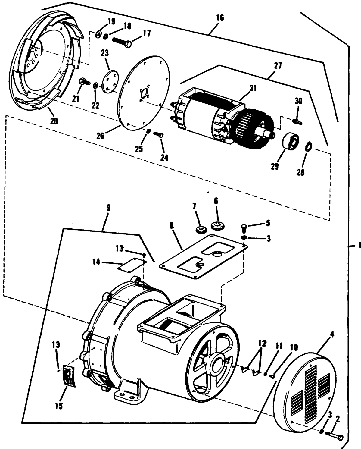
Figure 32. Generator Assembly (28 VDC, 60 Hz), Group 03 (Electrical Power Generation System)
