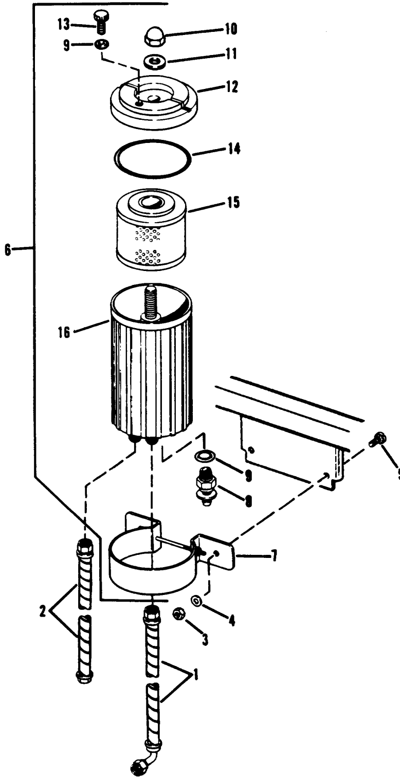
Figure 10. Fuel Filter/Water Separator, Group 04 (Fuel System and Oil Drain)
