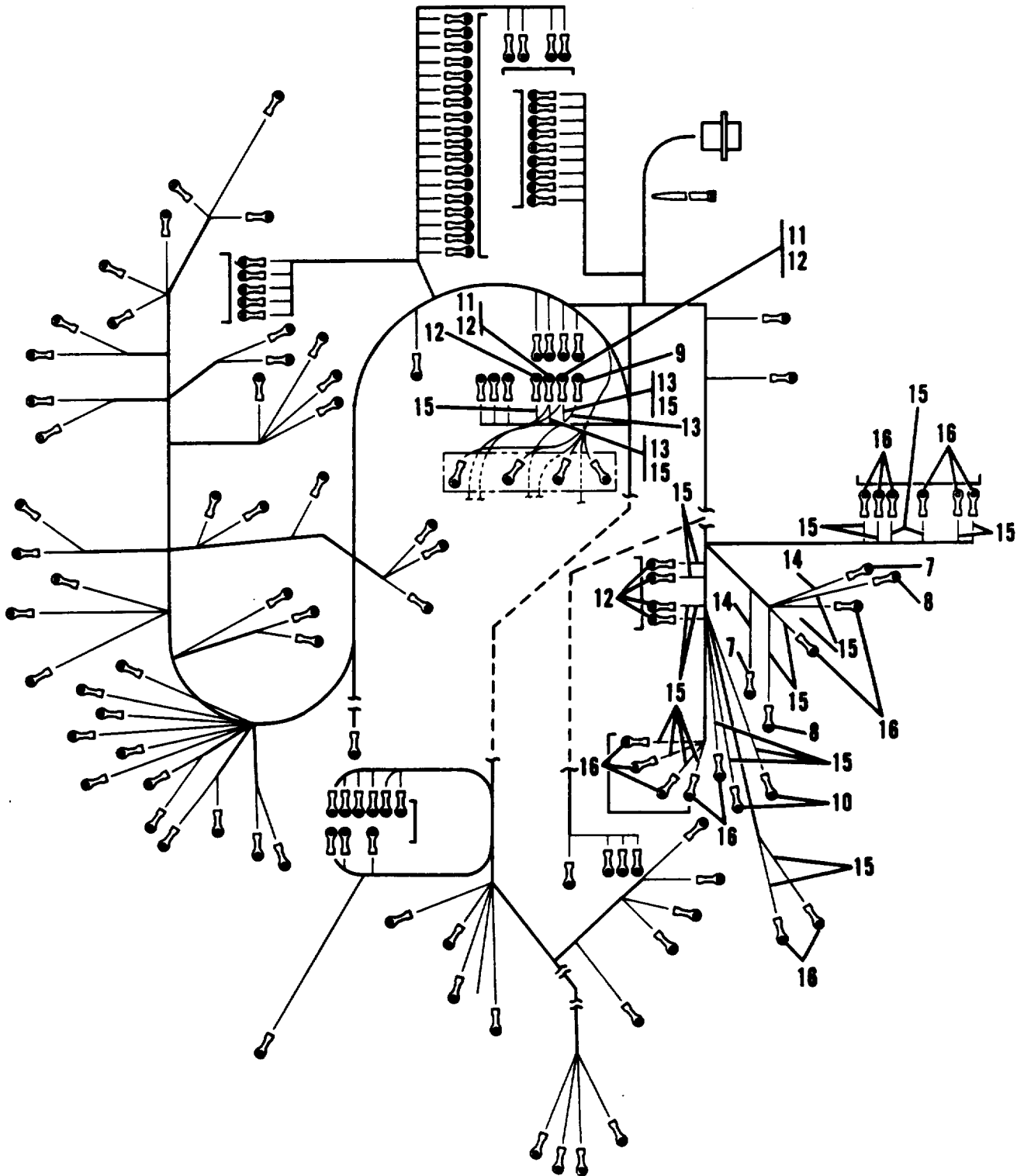
Figure 44. Control Wire Harness 60, 400 Hz, Group 08 (Generator Controls and Instruments) (Sheet 2 of 2)
