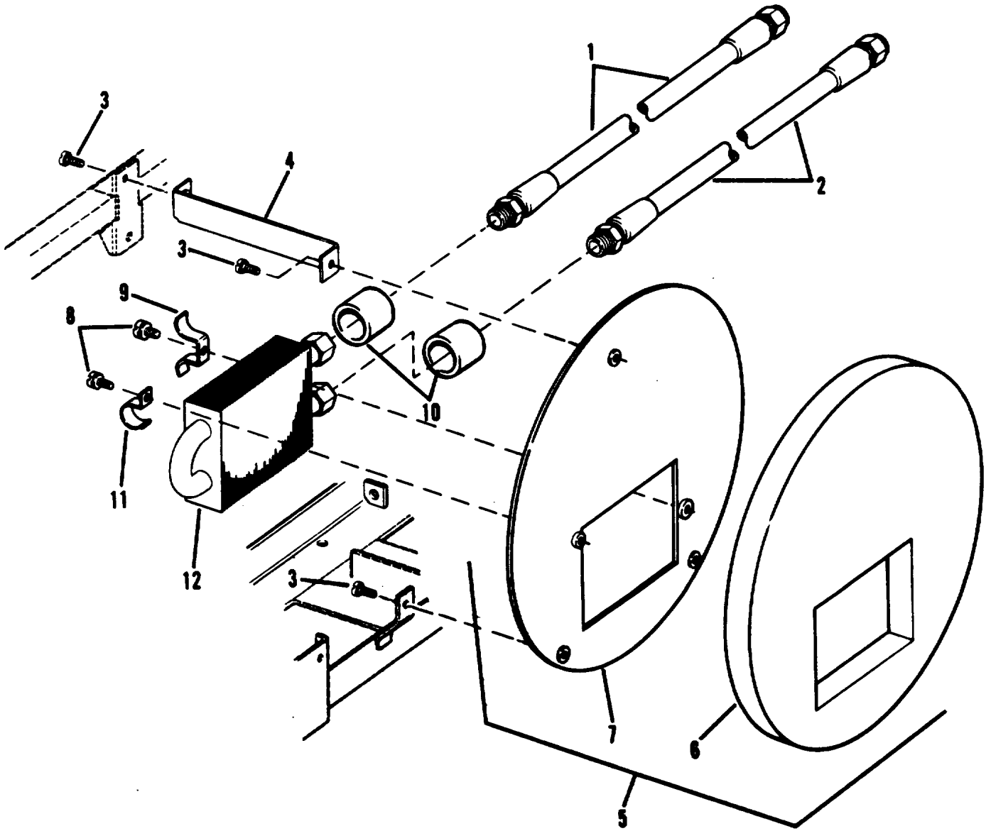
Figure 8. Oil Cooler, Group 05 (Engine)
