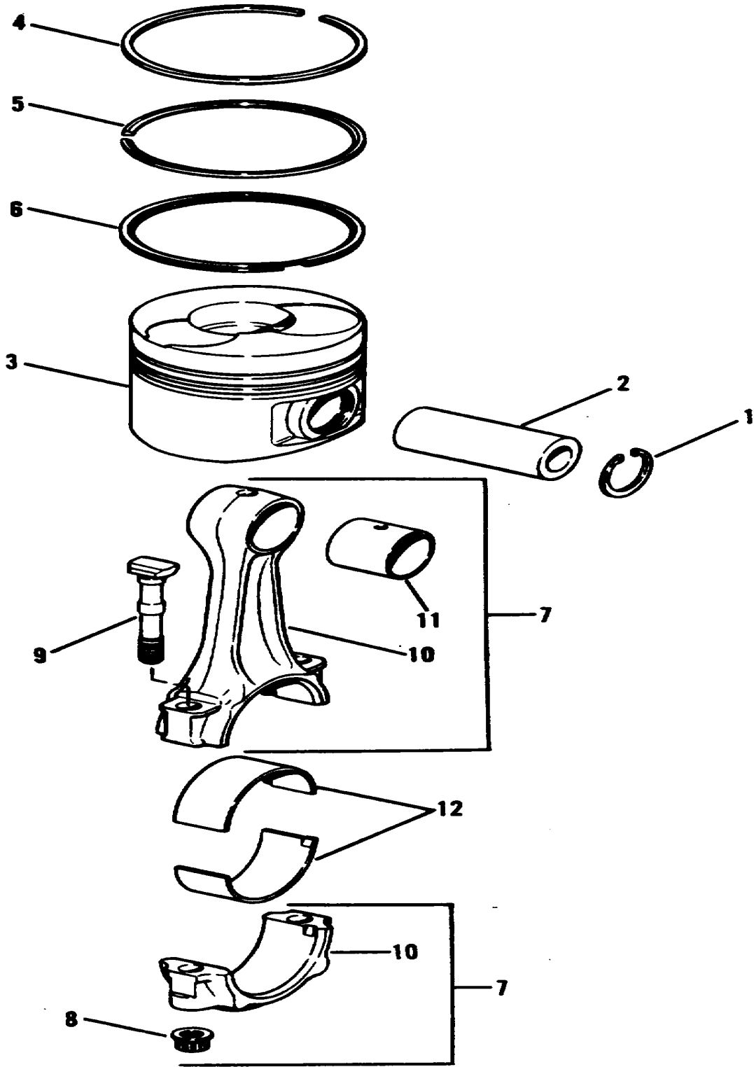
Figure 28. Connecting Rod and Piston, Group 05 (Engine)
