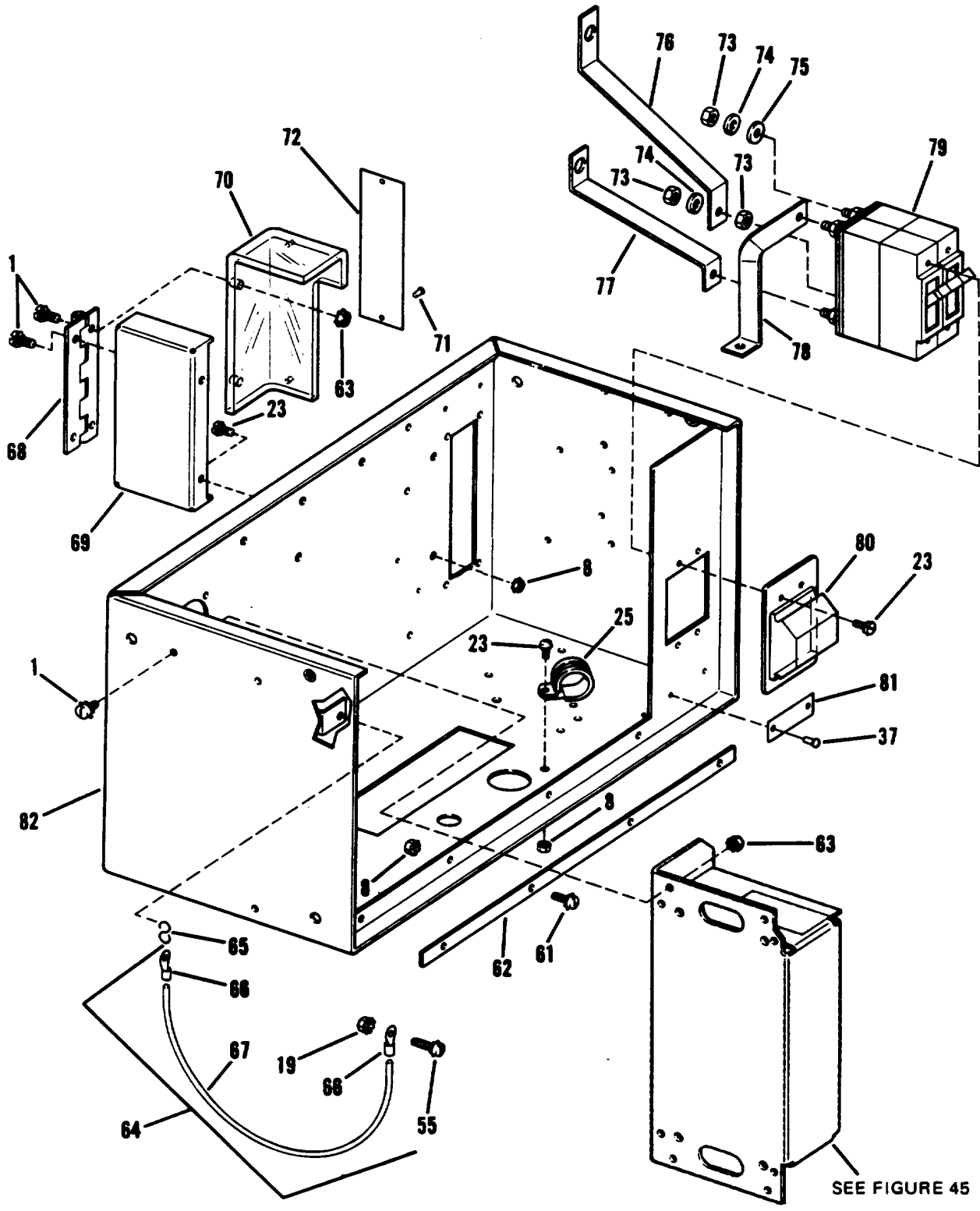
Figure 37. Generator Control Assembly 28 VDC, Group 08 (Generator Controls and Instruments) (Sheet 3 of 3)
