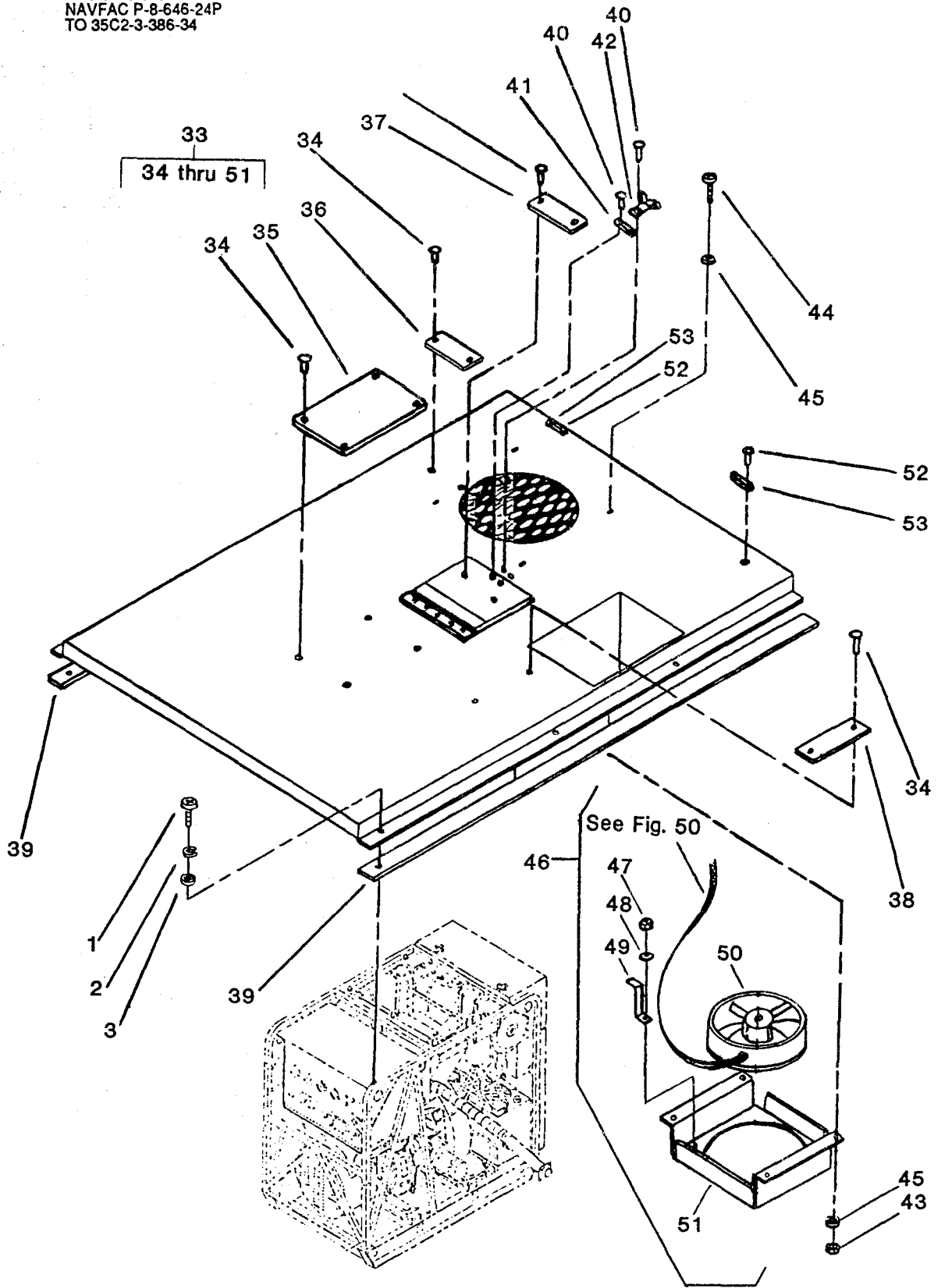
Figure 49. Panels, Group 10 (Sheet 4 of 7).
