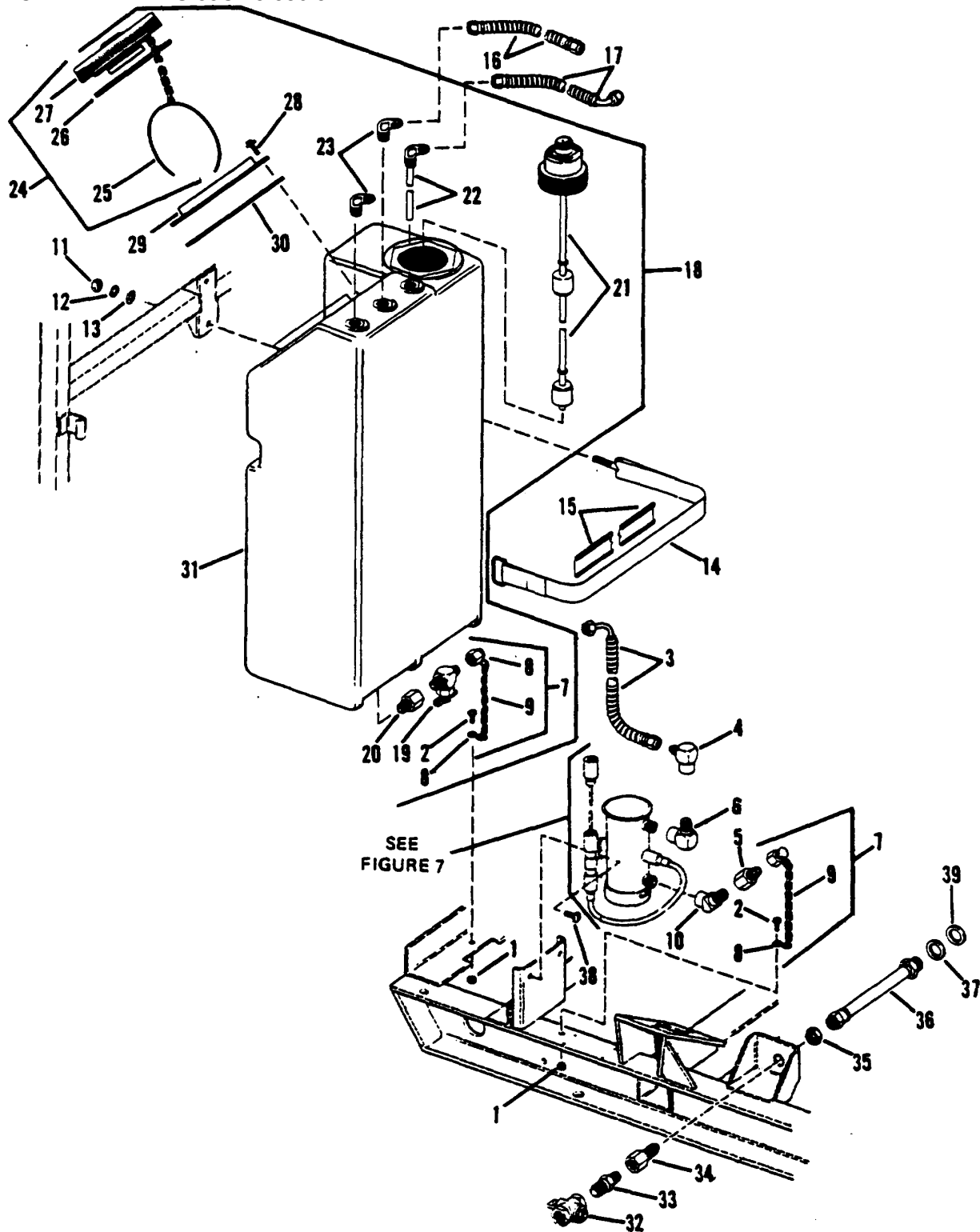
Figure 6. Fuel Tank, Lines and Oil Drain, Group 04 (Fuel System and Oil Drain)
