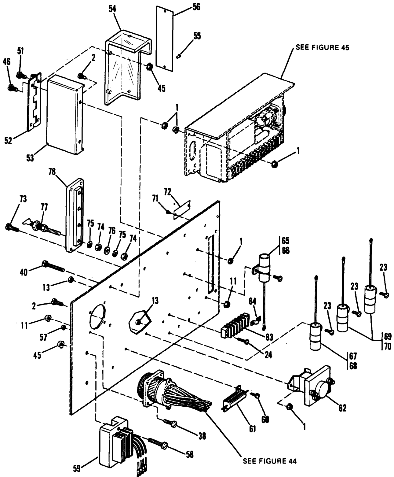
Figure 43. Generator Control Assembly 60, 400 Hz, Group 08 (Generator Controls and Instruments) (Sheet 3 of 3)
