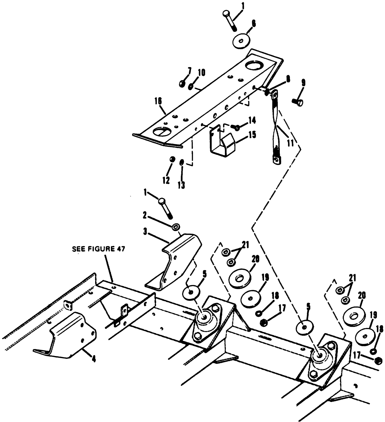
Figure 46. Engine Bracket and Generator Mount, Group 09 (Skid Base)
