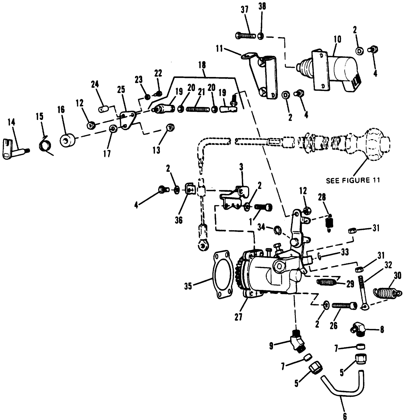
Figure 20. Governor and Fuel Shutdown Solenoid, Group 05 (Engine)
