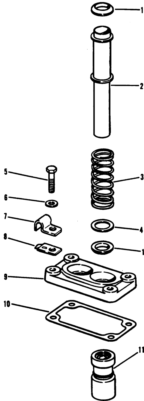
Figure 25. Push Rod Tube and Valve Tappet, Group 05 (Engine)
