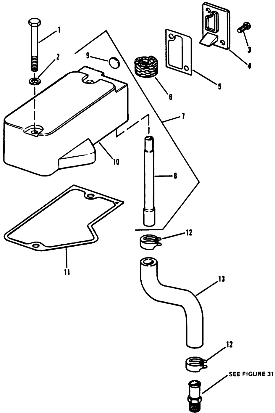
Figure 22. Rocker Arm Cover and Breather, Group 05 (Engine)
