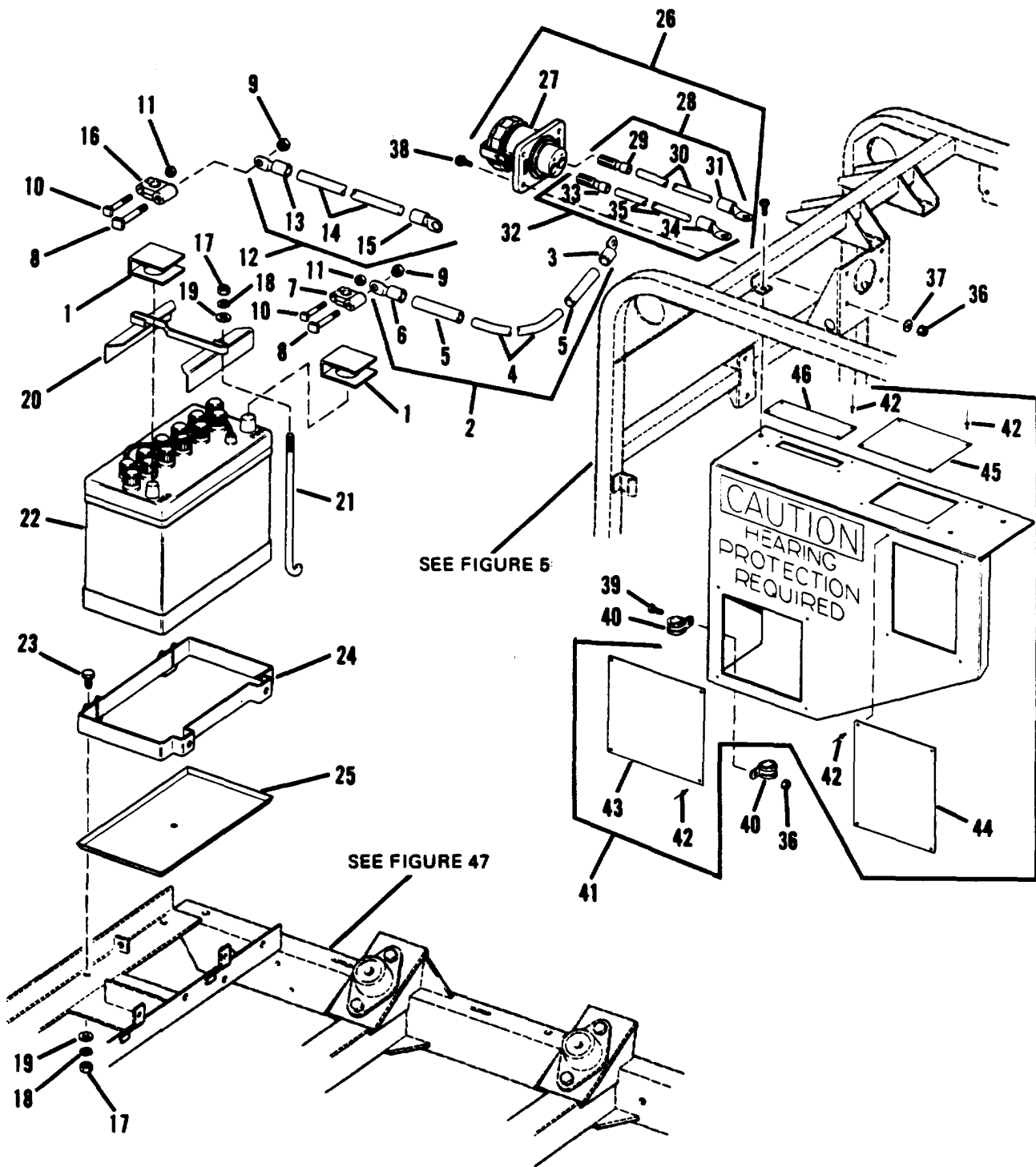
Figure 4. Battery, Battery Cables and Receptacle, Group 01 (DC Electrical and Control System)
