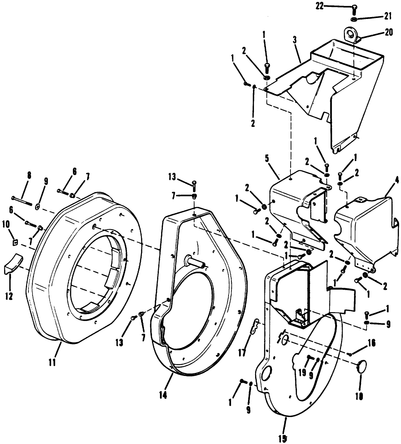
Figure 13. Engine Covers and Air Scroll, Group 05 (Engine)
