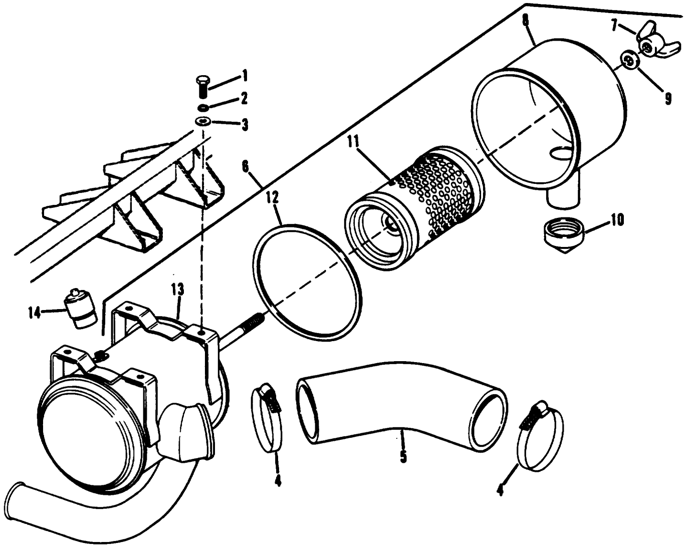
Figure 9. Air Intake Filter, Group 05 (Engine)
