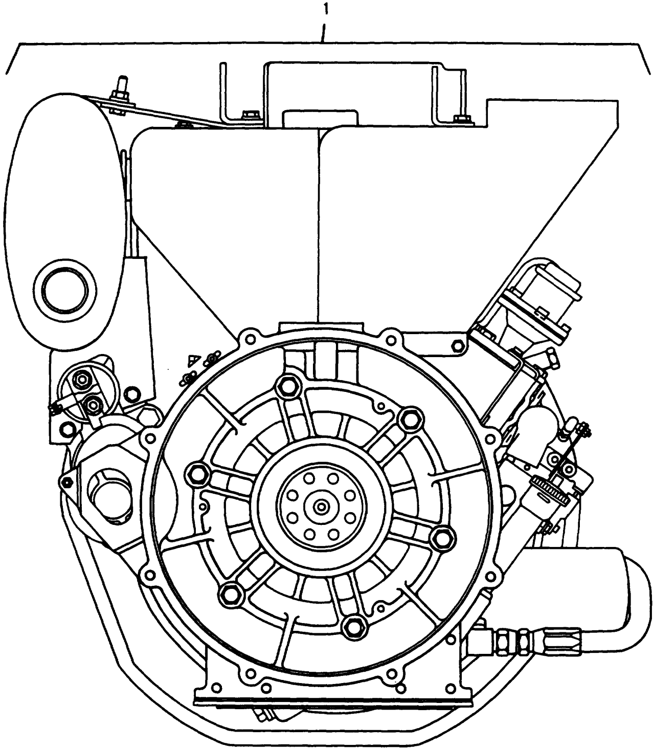
Figure 12. 3KW Diesel Engine, Group 05 (Engine)
