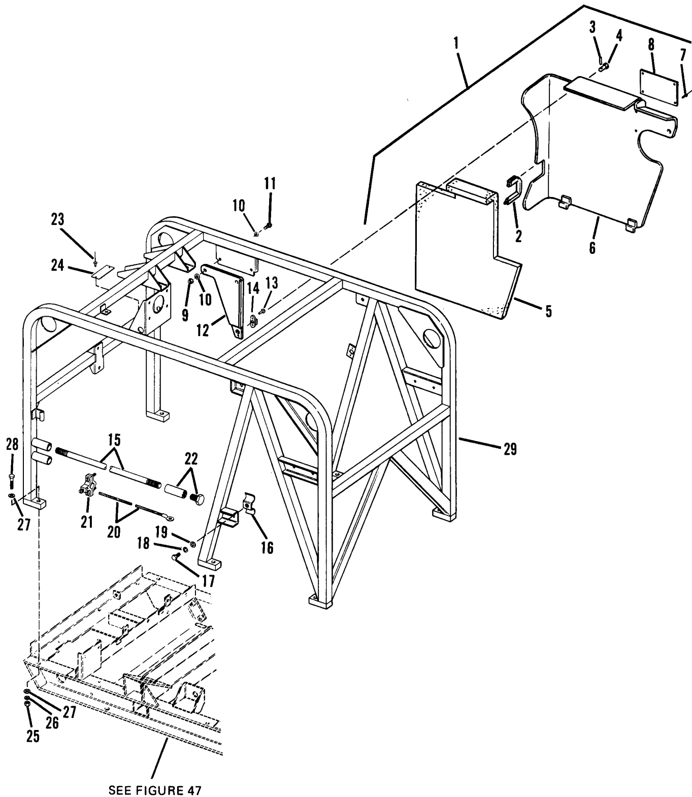
Figure 5. Frame, Ground Assembly and Guard, Group 02 (Frame)
