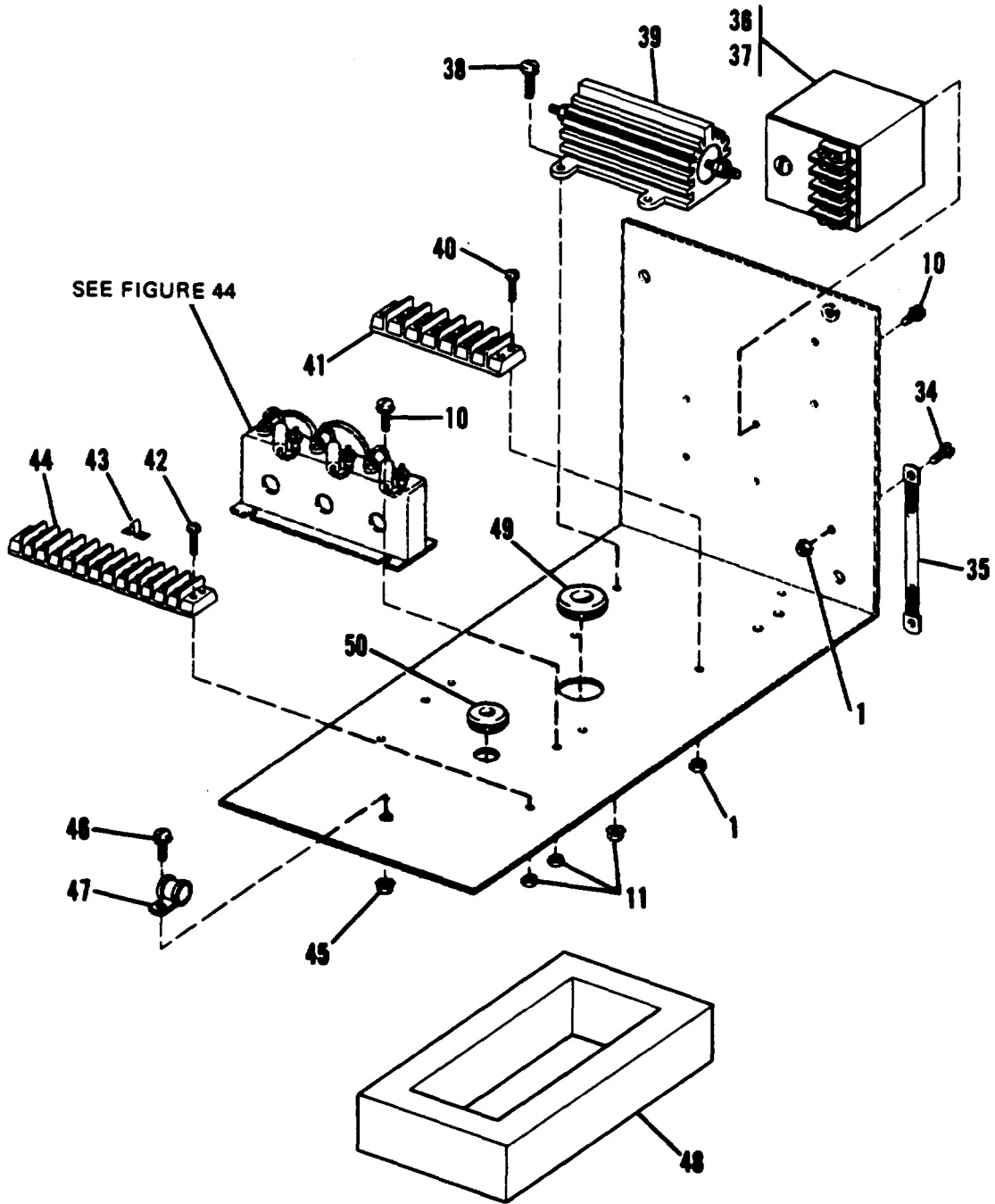
Figure 43. Generator Control Assembly 60, 400 Hz, Group 08 (Generator Controls and Instruments) (Sheet 2 of 3)
