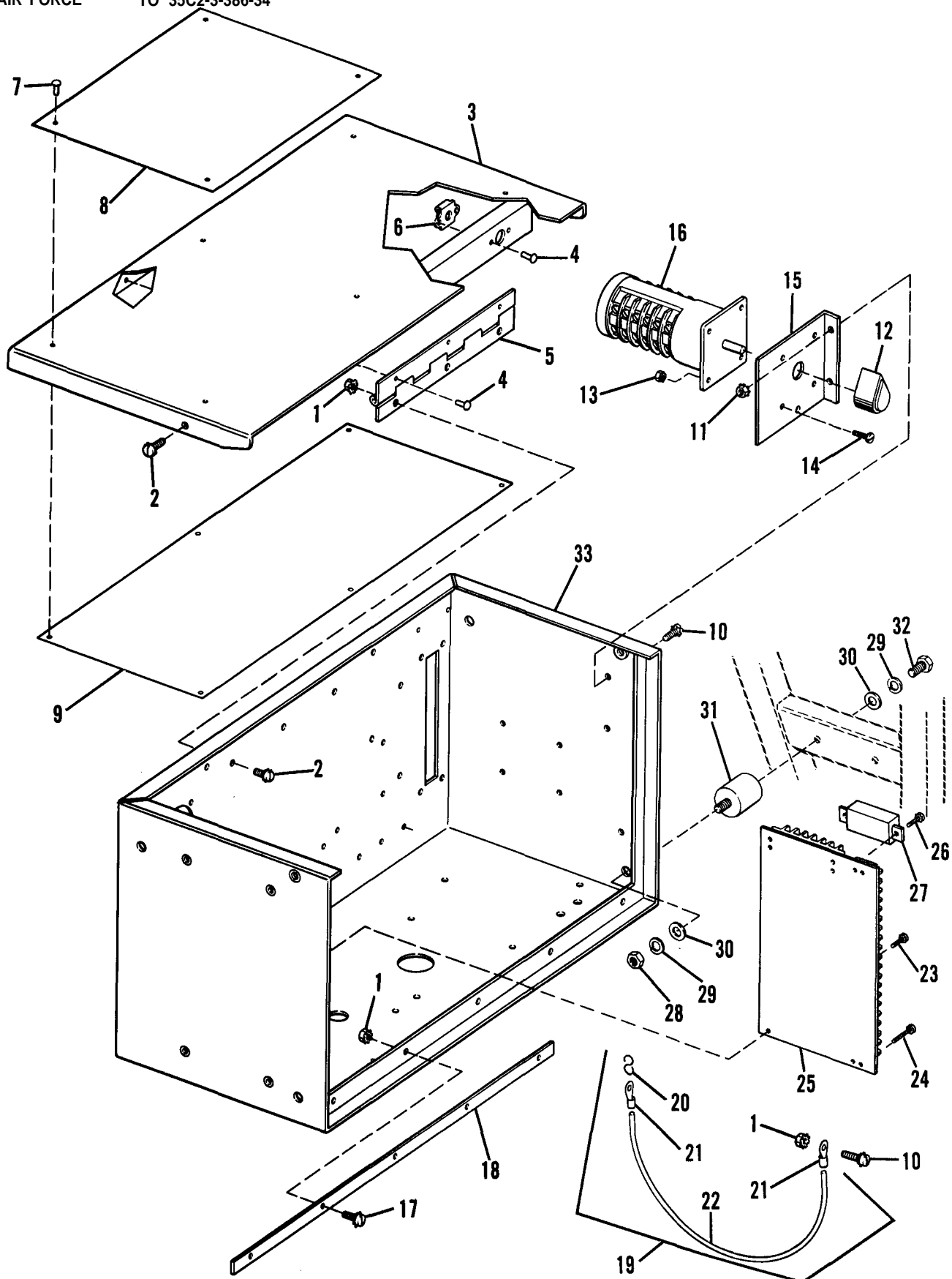
Figure 43. Generator Control Assembly 60,400 Hz, Group 08 (Generator Controls and Instruments) (Sheet 1 of 3)
