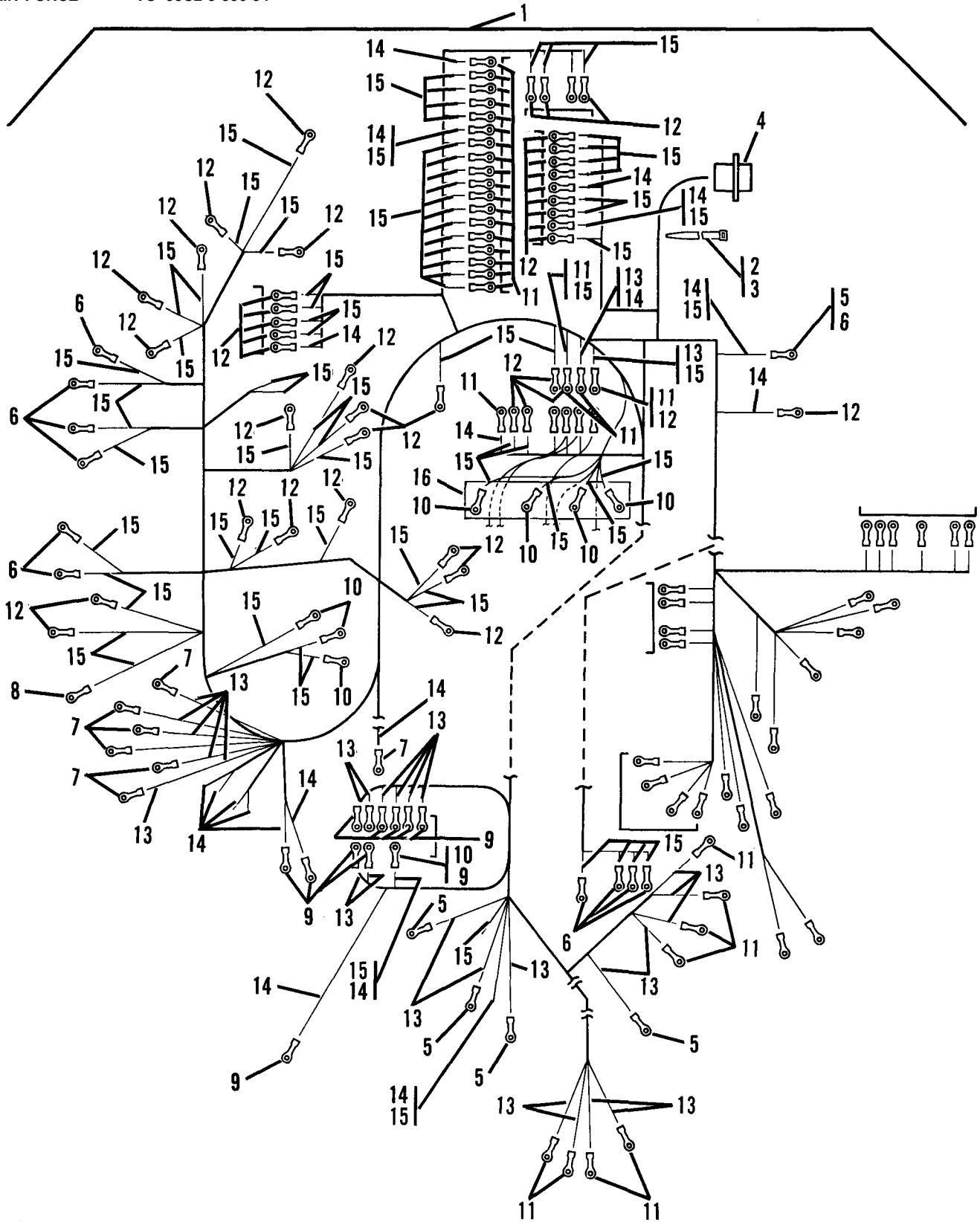
Figure 44. Control Wire Harness 60,400 Hz, Group 08 (Generator Controls and Instruments) (Sheet 1 of 2)
